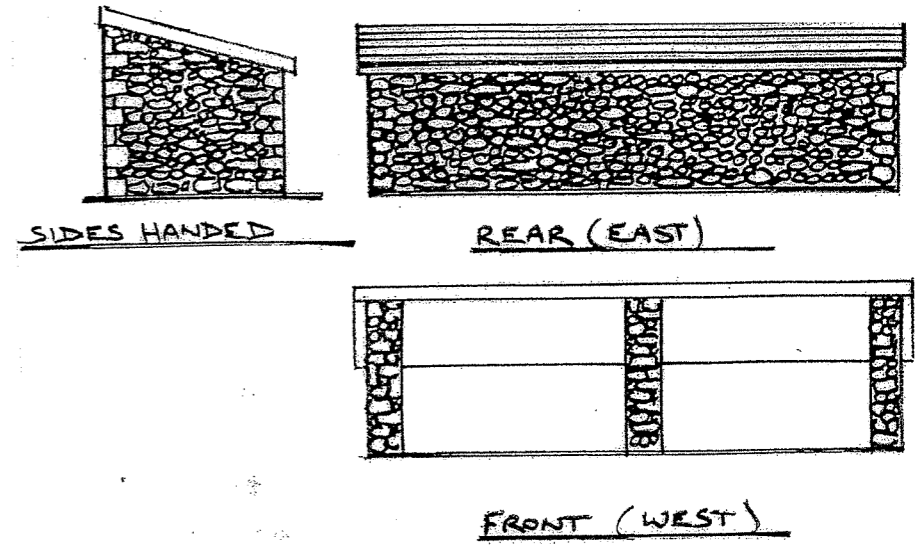
ELEVATIONS TO BIN STORE 1:100
