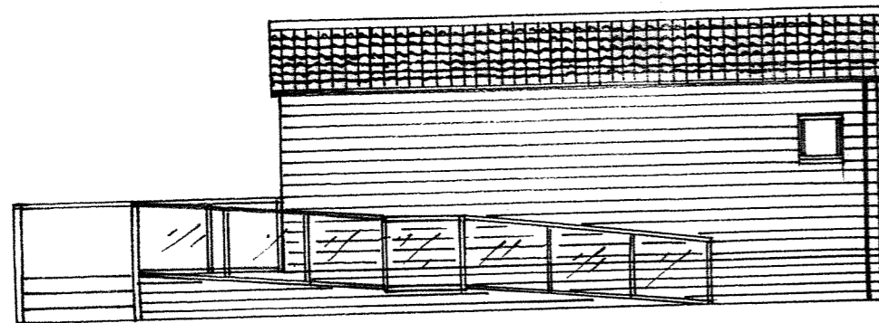
ELEVATIONS TO LODGES 1:100 0 1 2 3 4m
