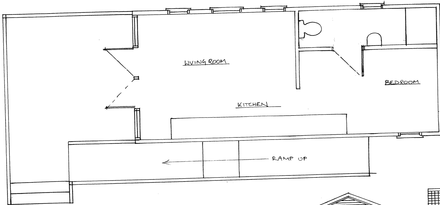
PLAN OF LODGES 1:50 0 1m 2m
